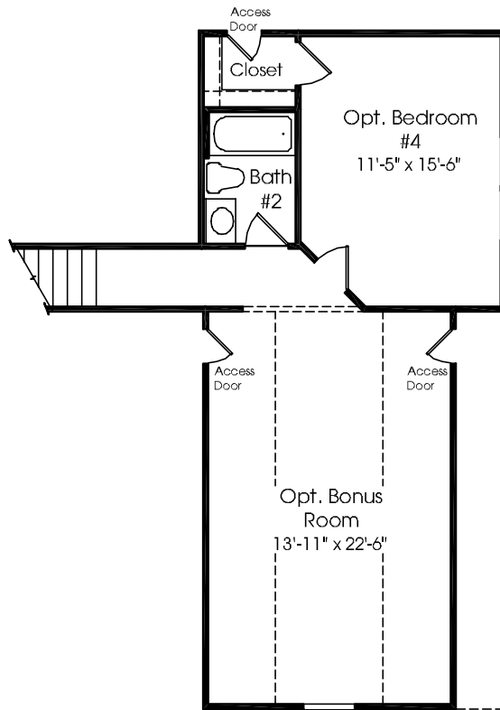
Opt. Bonus Room w/ Opt. Bedroom #4
