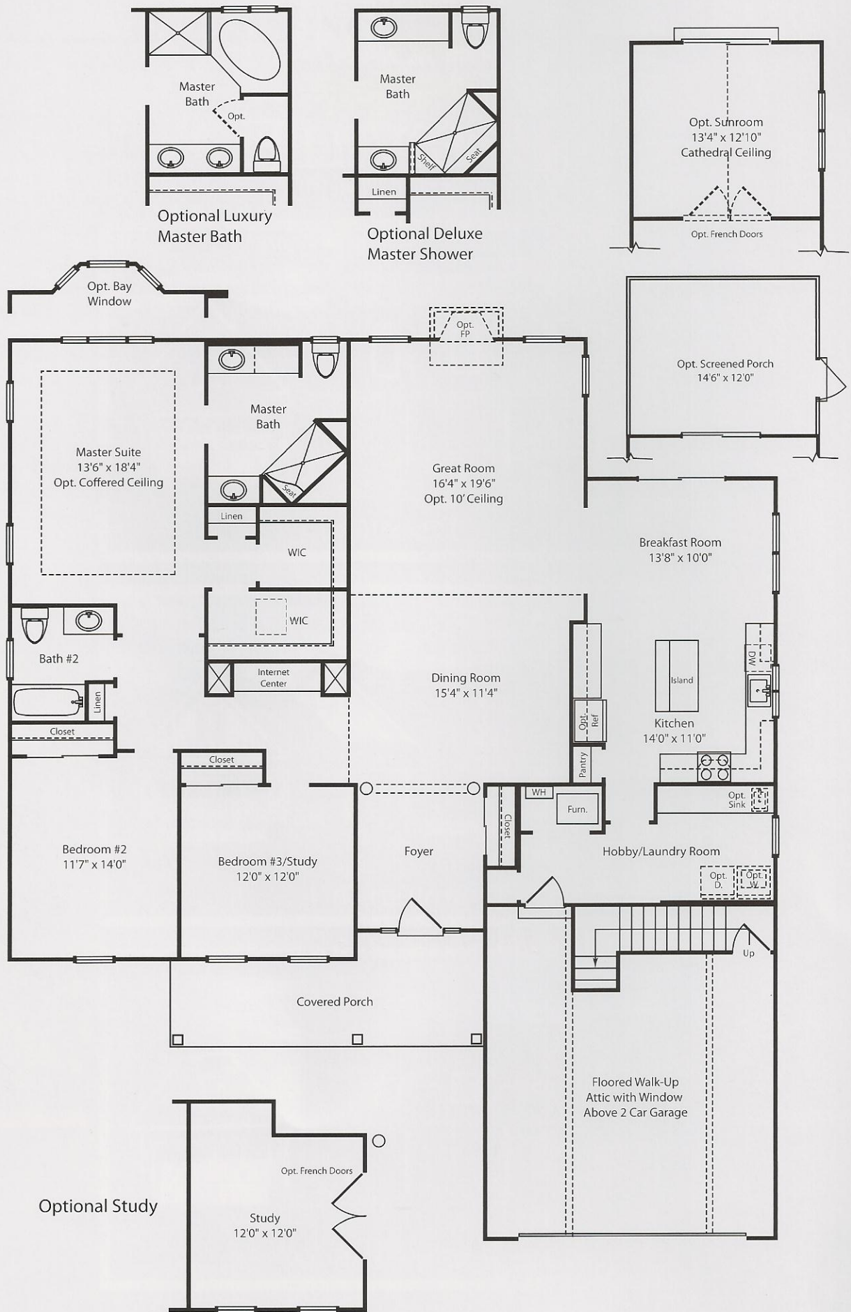
First Floor Plan Classic Elevation
