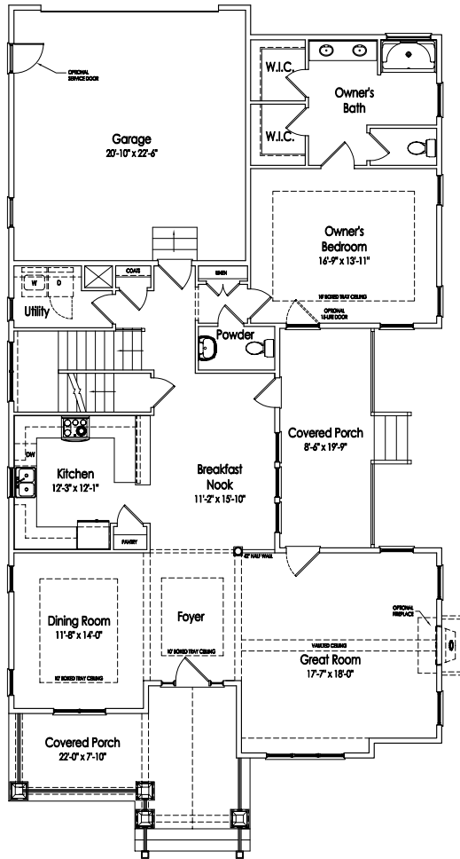
First Floor
