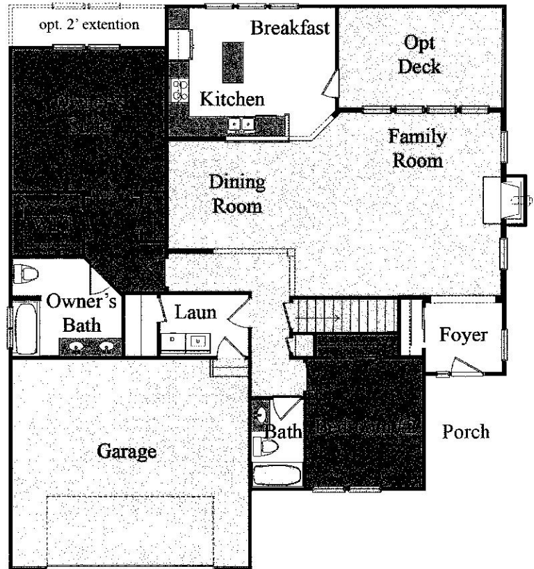
Dory First Floor Plan
